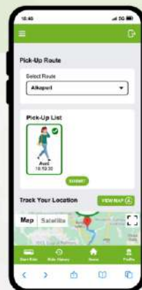
Driver Login
